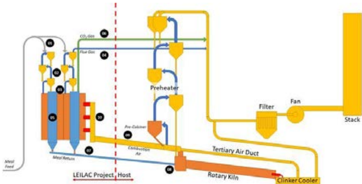
Figure 8 - Process Configuration
