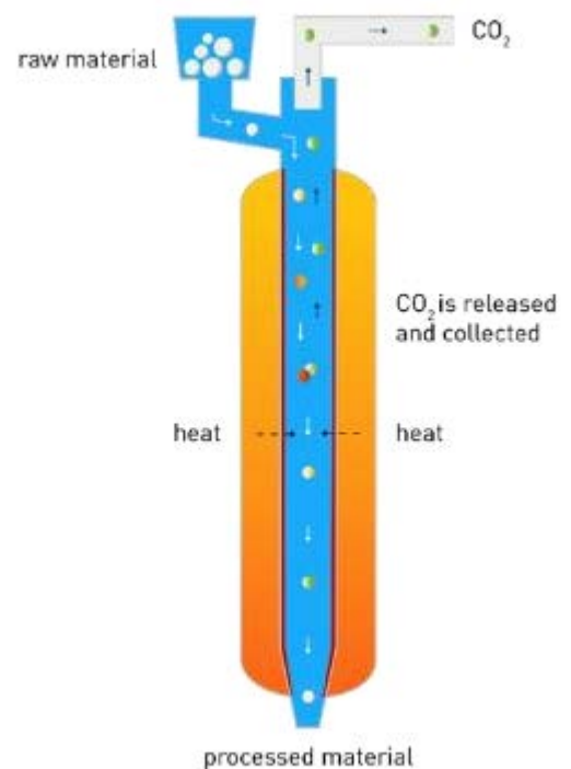
Figure 1 – LEILAC Technology design
