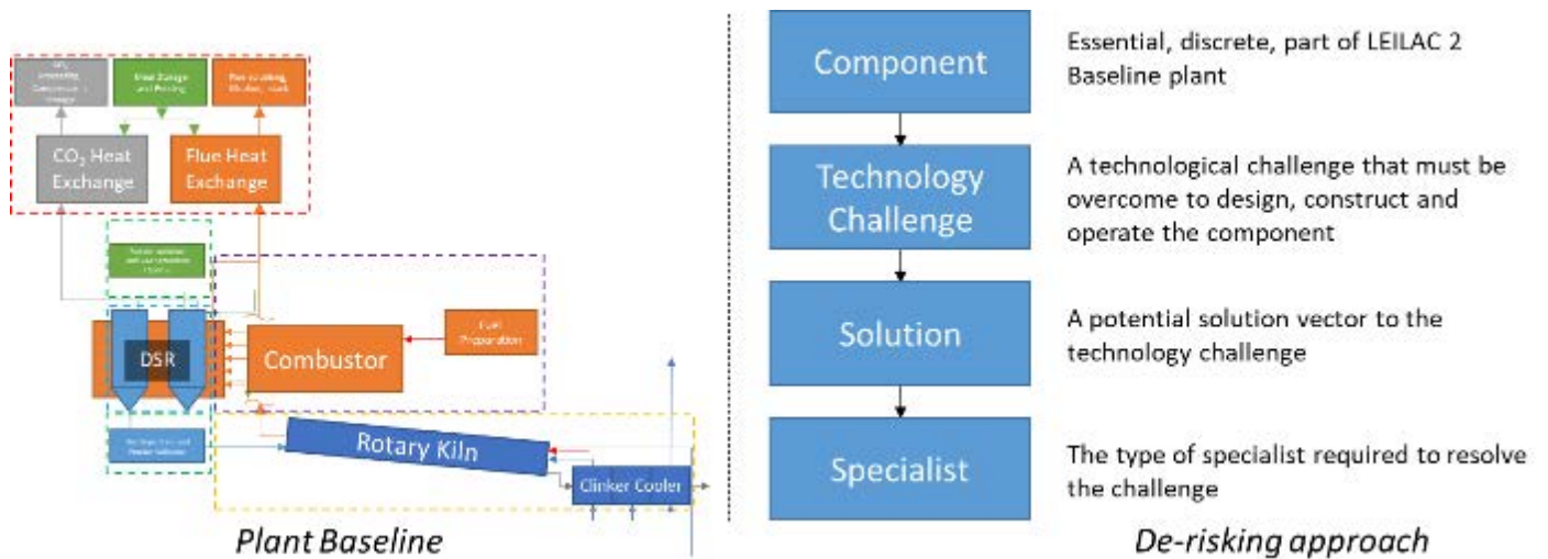
Figure 4 - System Components & Risk Identification Process
