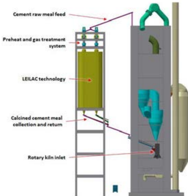
Figure 3 - Basis of Design (Tower Layout)
